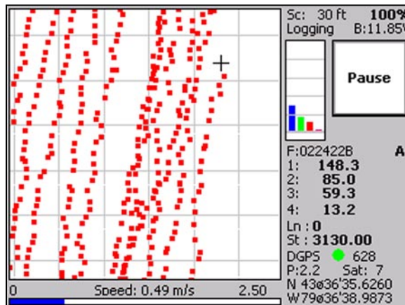
Figure 1.3: The NAV61MK2 in the Navigation mode
