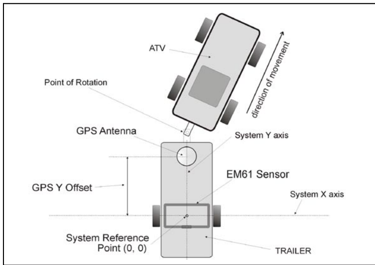
Figure 4.4: Geometry of the EM61-MK2 and GPS antenna during towing
