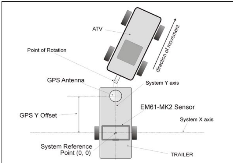
Figure 1.6: Geometry of the EM61 and GPS antenna during towing
