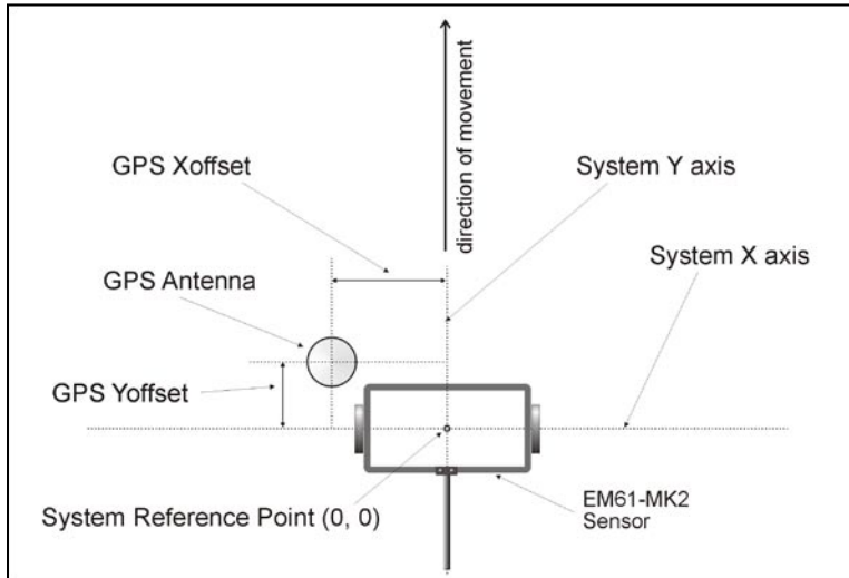
Figure 1.5: The NAV61MK2 system geometry
