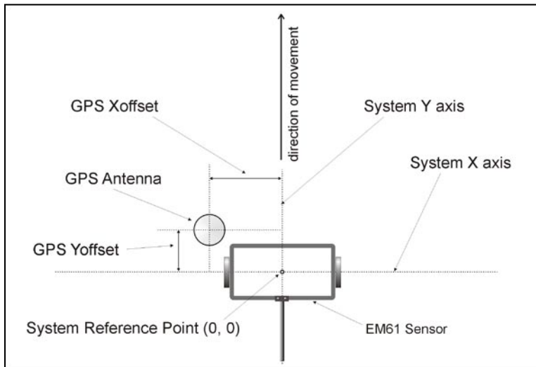
Figure 4.3: Geometry of the EM61-MK2 sensor and GPS in the field
