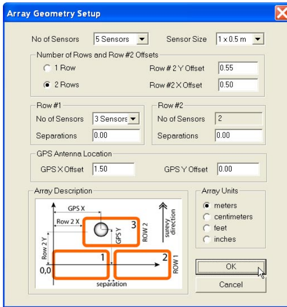
Figure 6.9: Array Geometry dialog with parameters for 2 rows, 5 sensors, and GPS antenna
