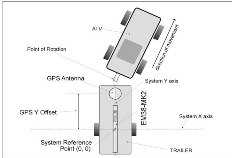
Figure 4.4: Geometry of the EM38-MK2 and GPS antenna during towing
