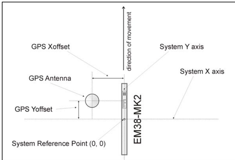
Figure 1.7: The NAV38MK2 system geometry
