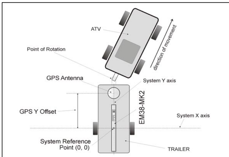
Figure 1.8: The NAV38MK2 system geometry for trailer mounted EM38-MK2
